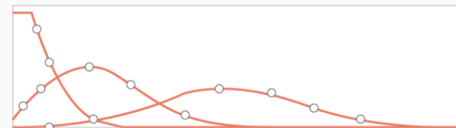
Poisson distribution
